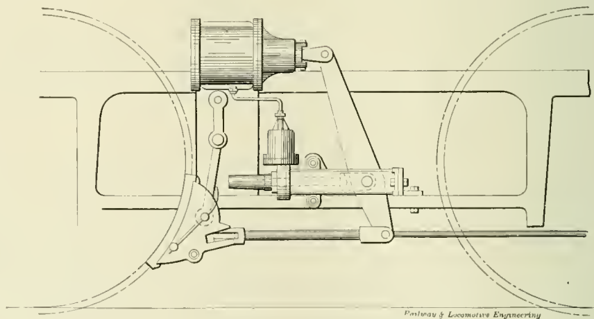
SLACK ADJUSTER ON DRIVER BRAKES.
